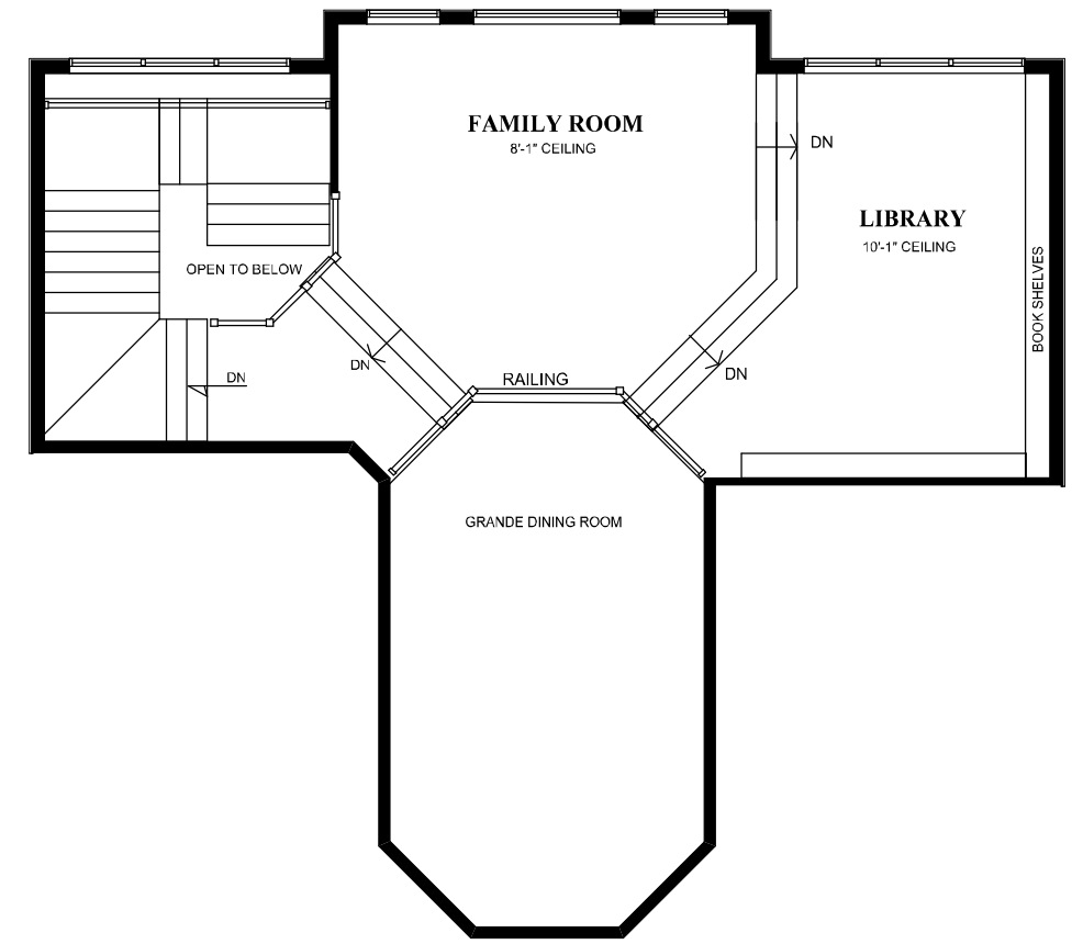
LOFT PLAN 550 SQ. FT.
