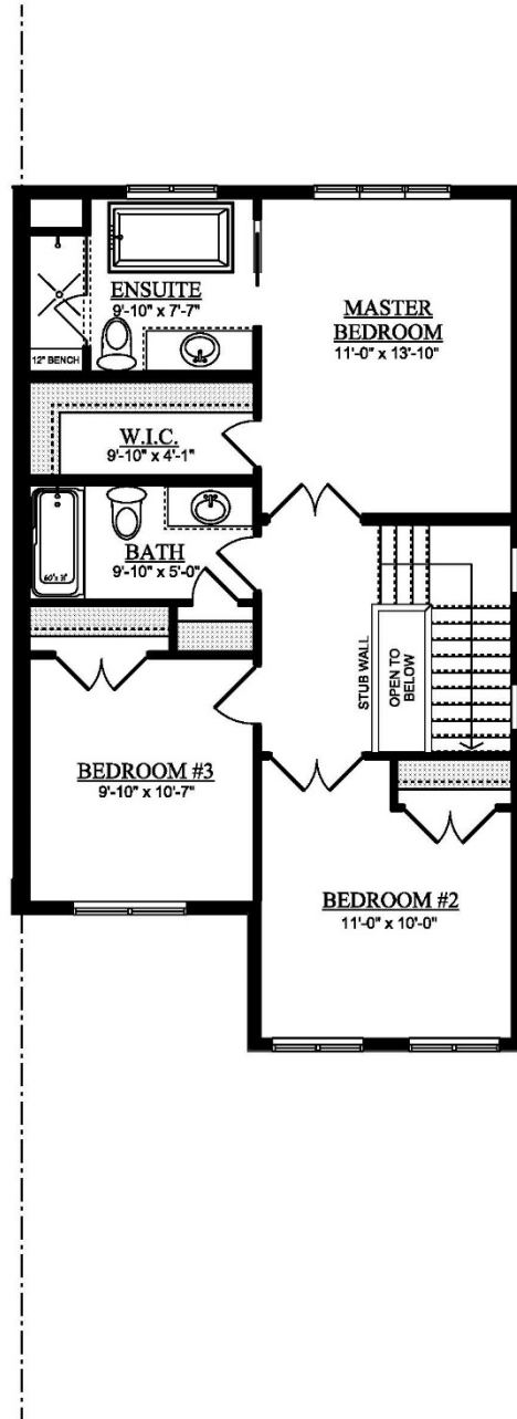
SECOND FLOOR PLAN 773 SQ. FT.
