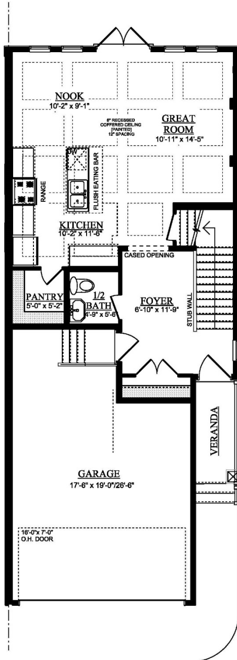
MAIN FLOOR PLAN 668 SQ. FT.
