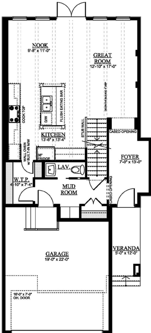
MAIN FLOOR PLAN 832 SQ. FT.
