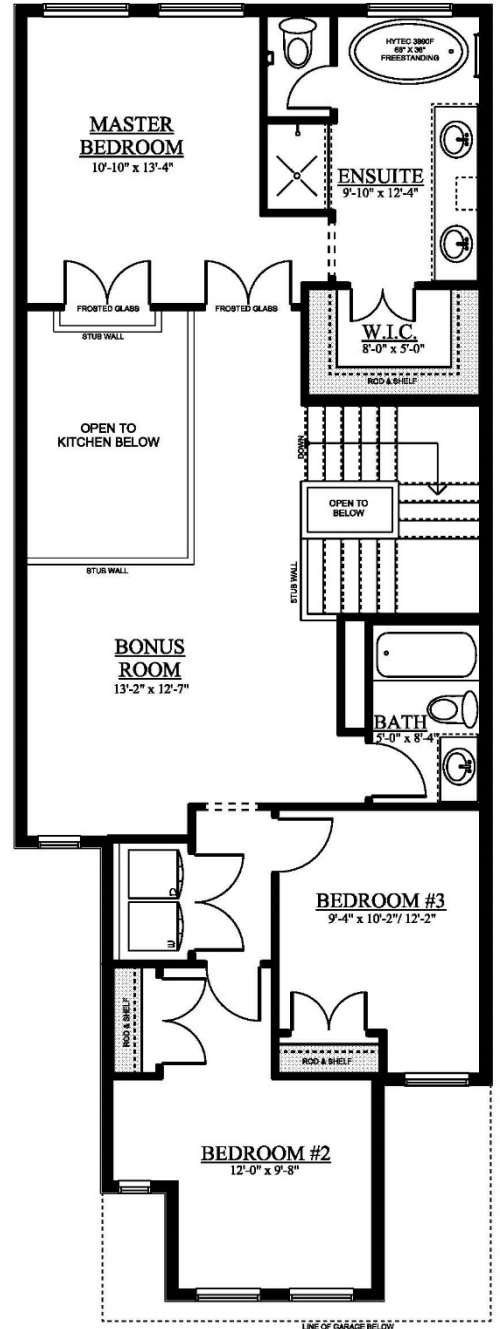
SECOND FLOOR PLAN 1083 SQ. FT.
