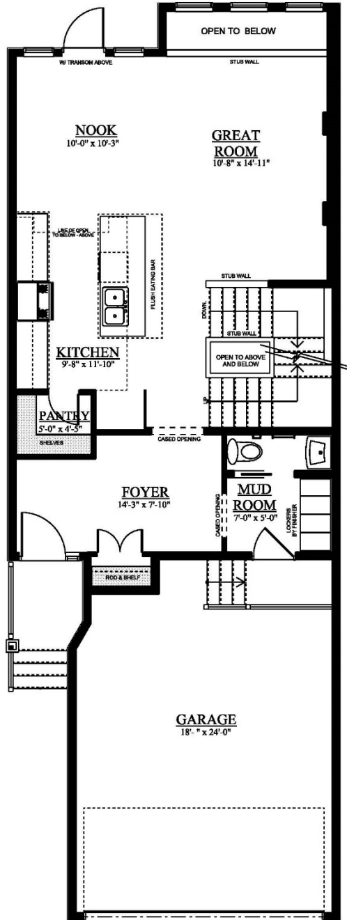
MAIN FLOOR PLAN 756 SQ. FT.
