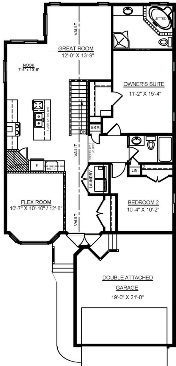
MAIN FLOOR PLAN 1364 SQ FT
