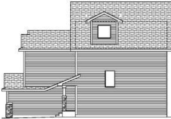
RIGHT ELEVATION "D"
