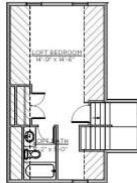
OPTIONAL LOFT DEVELOPMENT "F" 479 SQ FT
