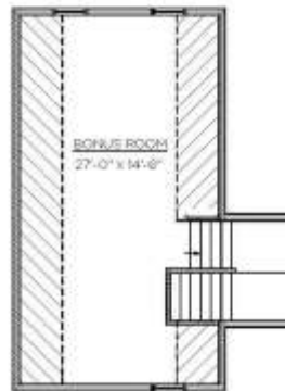
OPTIONAL LOFT DEVELOPMENT "D" 479 SQ FT
