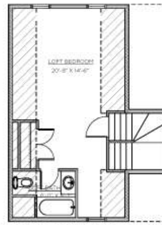
OPTIONAL LOFT DEVELOPMENT "F" 479 SQ FT
