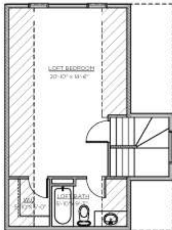
OPTIONAL LOFT DEVELOPMENT "E" 479 SQ FT
