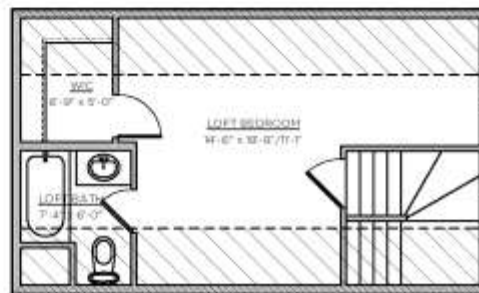
OPTIONAL LOFT DEVELOPMENT "C" 405 SQ FT
