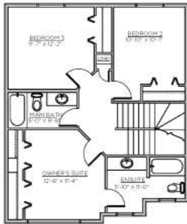
SECOND FLOOR PLAN 718 SQ FT
