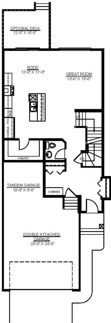
Main Floor 932 Sq. Ft
